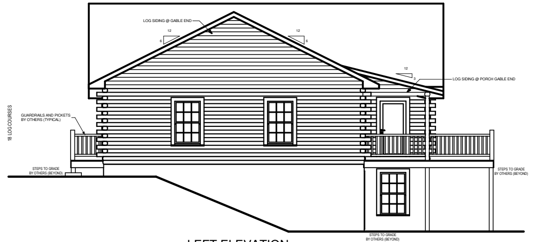
LEFT ELEVATION
