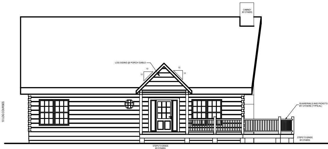
LEFT ELEVATION
