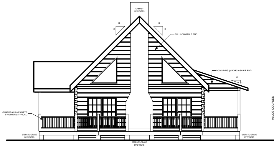
FRONT ELEVATION
