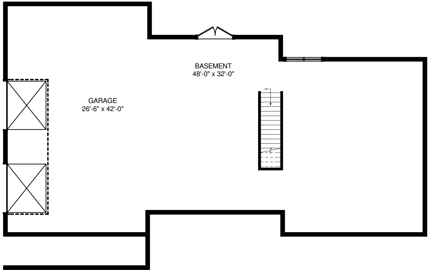
BASEMENT PLAN
