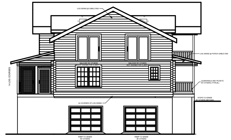
LEFT ELEVATION
