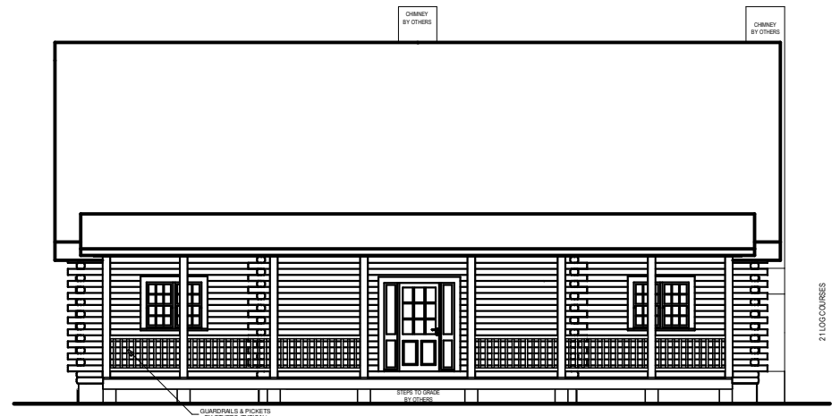
FRONT ELEVATION
