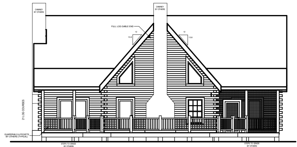
REAR ELEVATION
