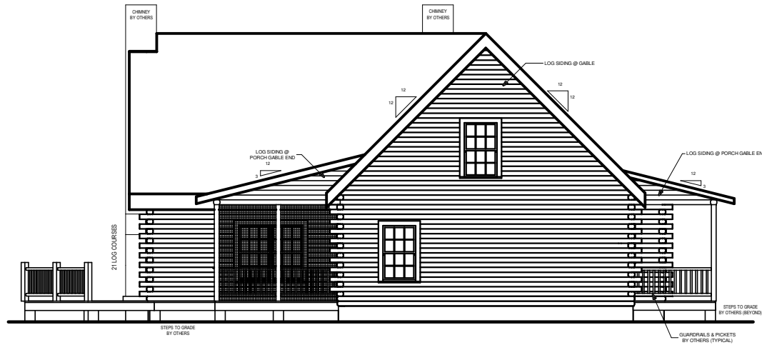
LEFT ELEVATION
