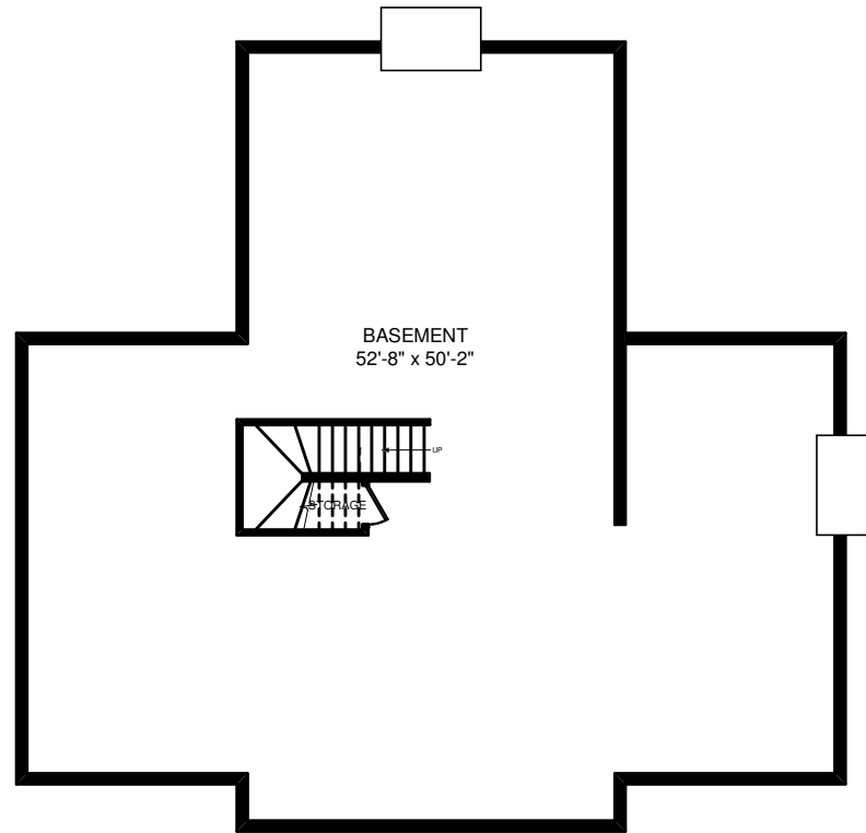
BASEMENT PLAN
