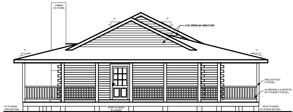
LEFT ELEVATION
