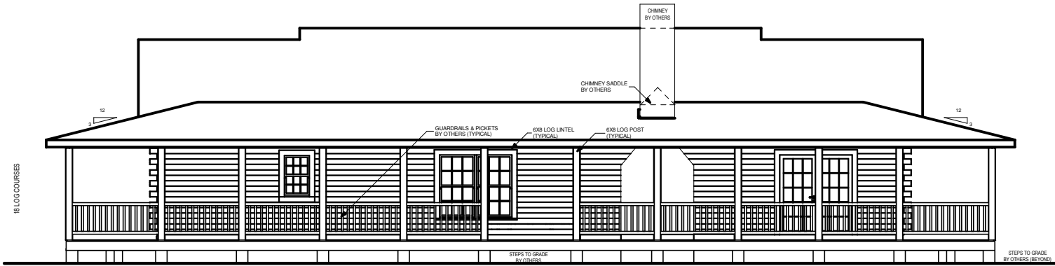
REAR ELEVATION
