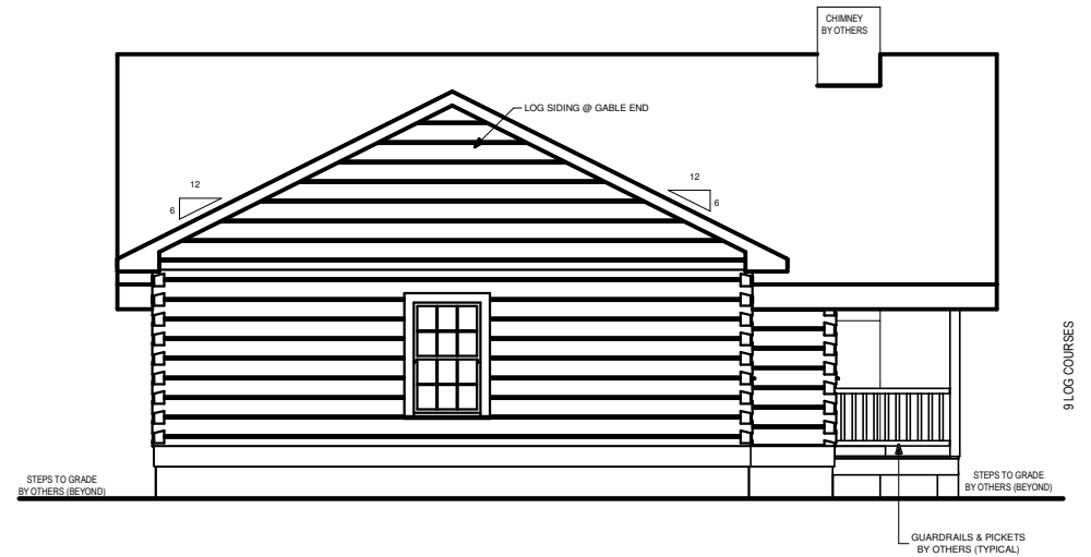
LEFT ELEVATION
